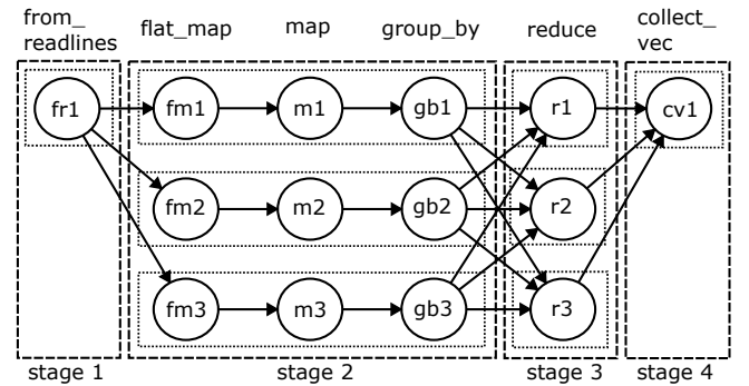
Figure 1: Dataflow graph for the word count example.
