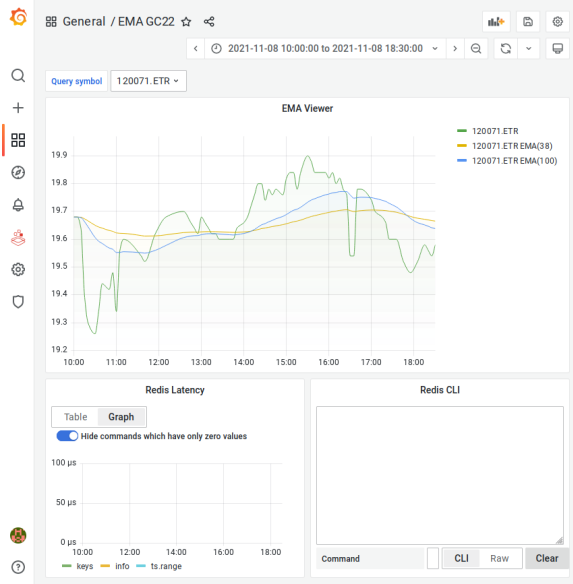
Figure 3: Smart visualization feature using Grafana.
