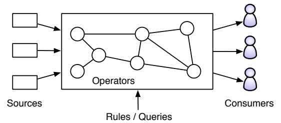
Figure 1: Abstract Model of Stream Processing Systems
